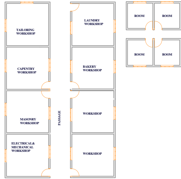
COLLEGE BLOCK FLOOR LAYOUT PLAN
